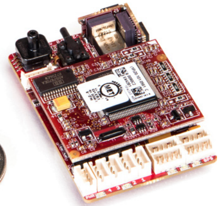
Kestrel Autopilot v2.4 2" x 1.37" x .47" 17 grams
